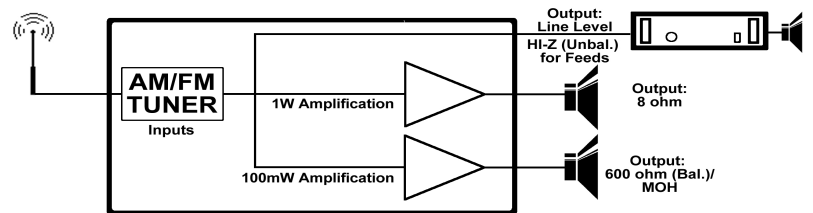
T118 Digital Tuner
